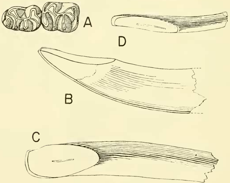
FIG. 7. Copemys toxodon , U.S.N.M. No. 1204, \times 10 . A, RM_{1-2} ; B, medial view of right lower incisor; C, ventral view of right upper incisor; D, dorsal view of another right lower incisor with same number.
